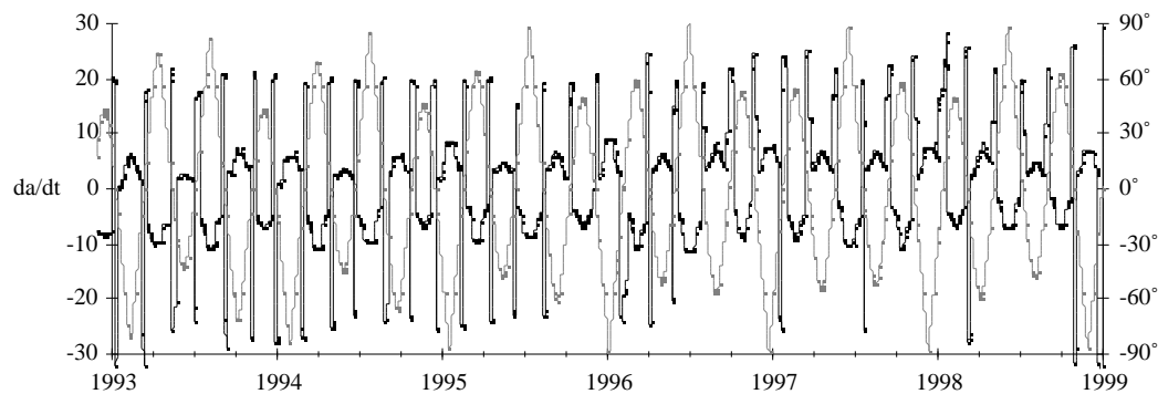
Figure 3. Change of a due to Anomalous Force. Solid line: da/dt , cm/day (left scale); Dotted Line: \delta (right scale).
